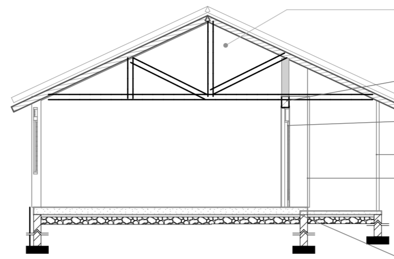
SECTION M-M
